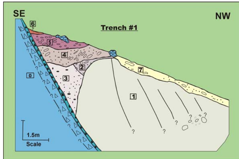
Fig.4: On the top of the figure the trench log section with the seven identified sedimentary units is shown (see text for description of the units). On the left picture showing, the field location of the Trench #1.
