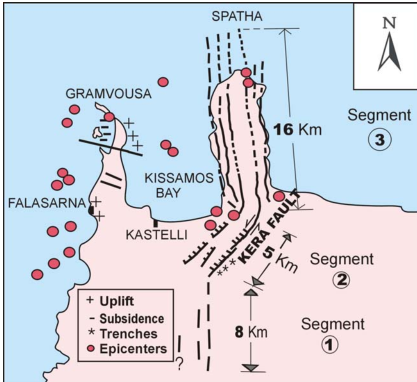
Fig. 3: Map showing the three segments of the active fault zone. Kera fault represents the shorter segment in the middle of the map, with a NE-SW orientation. The ascendent and descendent movements on Gramvousa peninsula are shown. Recent earthquake activity is also noted (1964-1999, M > 4.5 ) (after Mouslopoulou, 1999).
