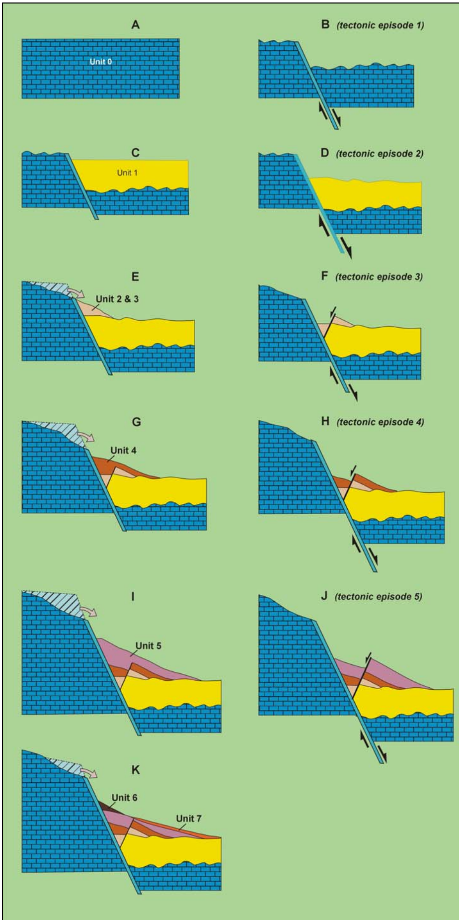
Fig 5: Retrodeformation of the Kera fault zone: A. Upper Cretaceous carbonate marine sedimentation. B. First tectonic episode. Formation of the Oligomictic breccia. C. Erosion of the fault scarp. Transgression and marly sedimentation (middle Miocene). D. Second tectonic episode. Formation of the polymictic breccia. E. Deposition of the first colluvial wedge. F. Third faulting event (post-Miocene time) (seismic event 3). G. Erosion and degradation of the fault scarp. Deposition of the second colluvial wedge. H. Fourth faulting event (Quaternary) (seismic event 4). I. Erosion of the fault scarp causes the deposition of the third colluvial wedge. J. Fifth faulting event (Quaternary) (seismic event 5). K. Deposition of the fourth colluvial wedge and formation of a thin soil horizon.
