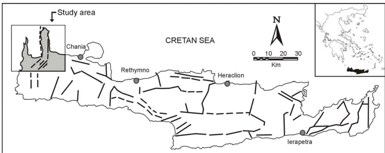
Fig.2: Simplified map showing the major fault zones on the island of Crete.
